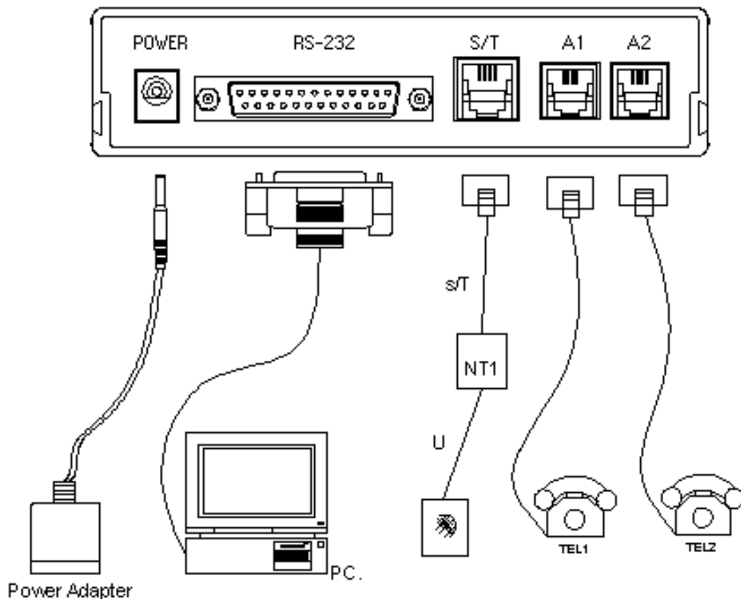
Fig 2-2 The rear panel of the TA
